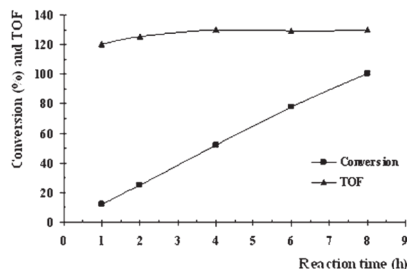
Figure 2. Kinetic profile and TOF value.
