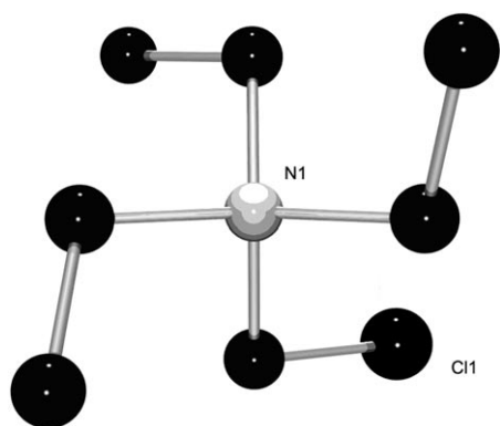
Figure 1. Ball-and-stick representation of [Et 3 NCH 2 Cl] + Cl − .
